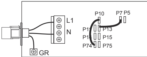
EXPORT Figure 6.0d 230V 50Hz Wiring
