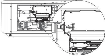
NORTH AMERICAN Figure 6.0c 240V 60Hz Wiring
