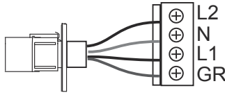
NORTH AMERICAN Figure 6.0c 240V 60Hz Wiring
