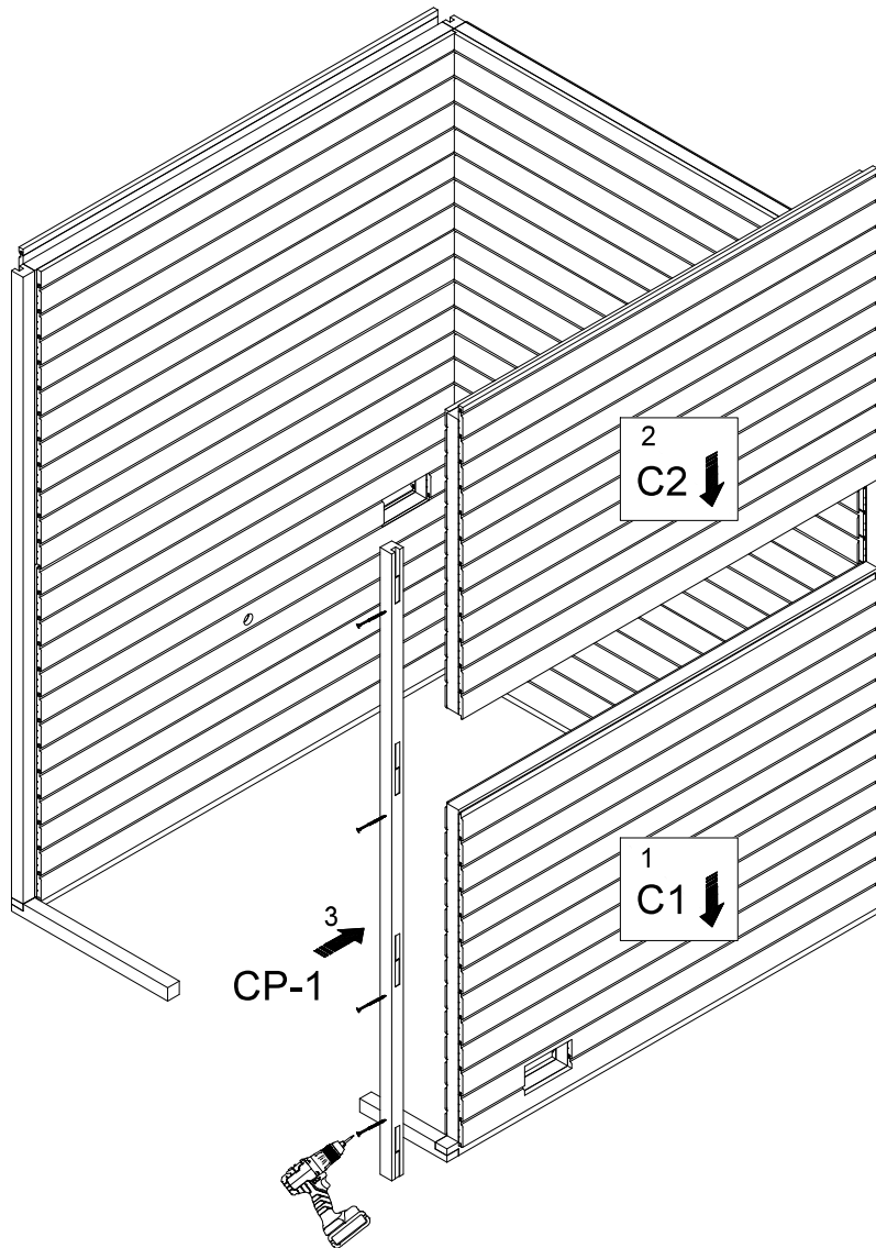
Figure 2.2b. Corner fixing
